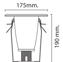
WL-5001BF-WH 220 W175xH190 mm E27=1x40W
