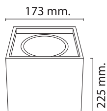
WL-5508BK/WH 440 W173xH225 mm E27=1x40W
