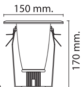
WL-P4012-B-4SC-G 150 W150xH170mm E27=1x40W
