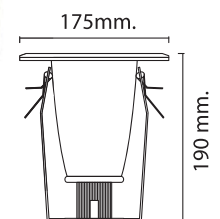
WL-P5001 5KG 160 W175xH190 mm E27=1x40W
