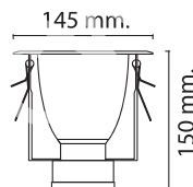
WL-4001BF-WH 170 W145xH150 mm E27=1x40W
