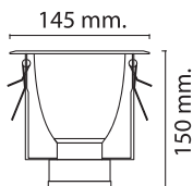
WL-3012-AF-WH 160 W145xH150 mm E27=1x40W
