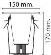
WL-P4001-4WH 76 W150xH170mm E27=1x40W
