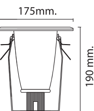
WL-P5001-5WH 130 W175xH190 mm E27=1x40W
