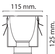
WL-3012A-SN/N 150 W115xH125 mm E27=1x40W ឧត្តមជ័យ
