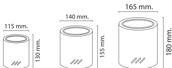
WL-5008WH 260 W165xH180 mm E27=1x40W
